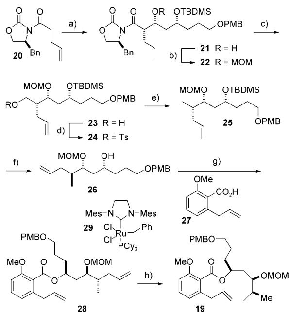
Scheme 5. Synthesis of the macrolactone 19 by Mitsunobu esterification and ring-closing metathesis. a) \text{TiCl}_4 (1.05 equiv), (–)-spartein (2.5 equiv), \text{CH}_2\text{Cl}_2 , 0^\circ\text{C} , add aldehyde 8 (1.1 equiv), 0^\circ\text{C} , 1 h, 68%; b) i\text{Pr}_2\text{NEt} (20 equiv), \text{MeOCH}_2\text{Cl} (10 equiv), \text{Bu}_4\text{NI} (0.1 equiv), 0 \rightarrow 23^\circ\text{C} , 3 d, 82%; c) \text{NaBH}_4 (5 equiv), \text{H}_2\text{O}/\text{THF} (1:2), 0 \rightarrow 23^\circ\text{C} , 12 h, 86%; d) \text{TsCl} (3 equiv), pyridine, 0^\circ\text{C} , 12 h, 95%; e) \text{Et}_3\text{BHLi} (3.6 equiv), THF, 0 \rightarrow 23^\circ\text{C} , 15 h, 95%; f) TBAF (3 equiv), THF, 0 \rightarrow 23^\circ\text{C} , 48 h, 99%; g) \text{Ph}_3\text{P} (2.5 equiv), acid 27 (5 equiv), DIAD (2.55 equiv), toluene, 23^\circ\text{C} , 3 h, 71%; h) Grubbs catalyst 29 (0.1 equiv), toluene, 70^\circ\text{C} , 2 h, 75% of ( E )- 19 and 12% of ( Z )- 19 . DIAD = diisopropylazodicarboxylate.
