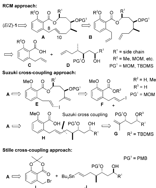
Scheme 2. General approaches to the macrolactone core of the salicylhalamides. RCM = ring-closing metathesis, MOM = methoxymethyl, TBDMS = tert -butyldimethylsilyl, PMB = para -methoxybenzyl.
