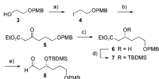
Scheme 3. Synthesis of the protected hydroxy aldehyde 8 . a) PPh 3 (1.01 equiv), imidazole (2 equiv), I 2 (1.01 equiv), THF, 0 °C, 1 h, 97%; b) NaH (1.2 equiv), ethyl acetoacetate, THF, n BuLi (1.2 equiv), -50 °C, 30 min, then add iodide 4 (1 equiv), 95%; c) [RuCl 2 (PhH)] 2 (0.003 equiv), ( R )-(+)-BINAP (0.07 equiv), DMF, 90 °C, 20 min, then add to 5 in EtOH, H 2 (4 bar), 90 °C, 20 h, 82%, 95% ee ; d) TBDMSOTf (1.12 equiv), 2,6-lutidine (2.5 equiv), CH 2 Cl 2 , 0–23 °C, 1 h, 100%; e) DIBAL (1.2 equiv), CH 2 Cl 2 , -78 °C, 2 h, 83%. BINAP = 2,2'-bis(diphenylphosphanyl)-1,1'-binaphthyl, TBDMSOTf = tert -butyldimethylsilyltriflate, DIBAL = diisobutylaluminum hydride.
